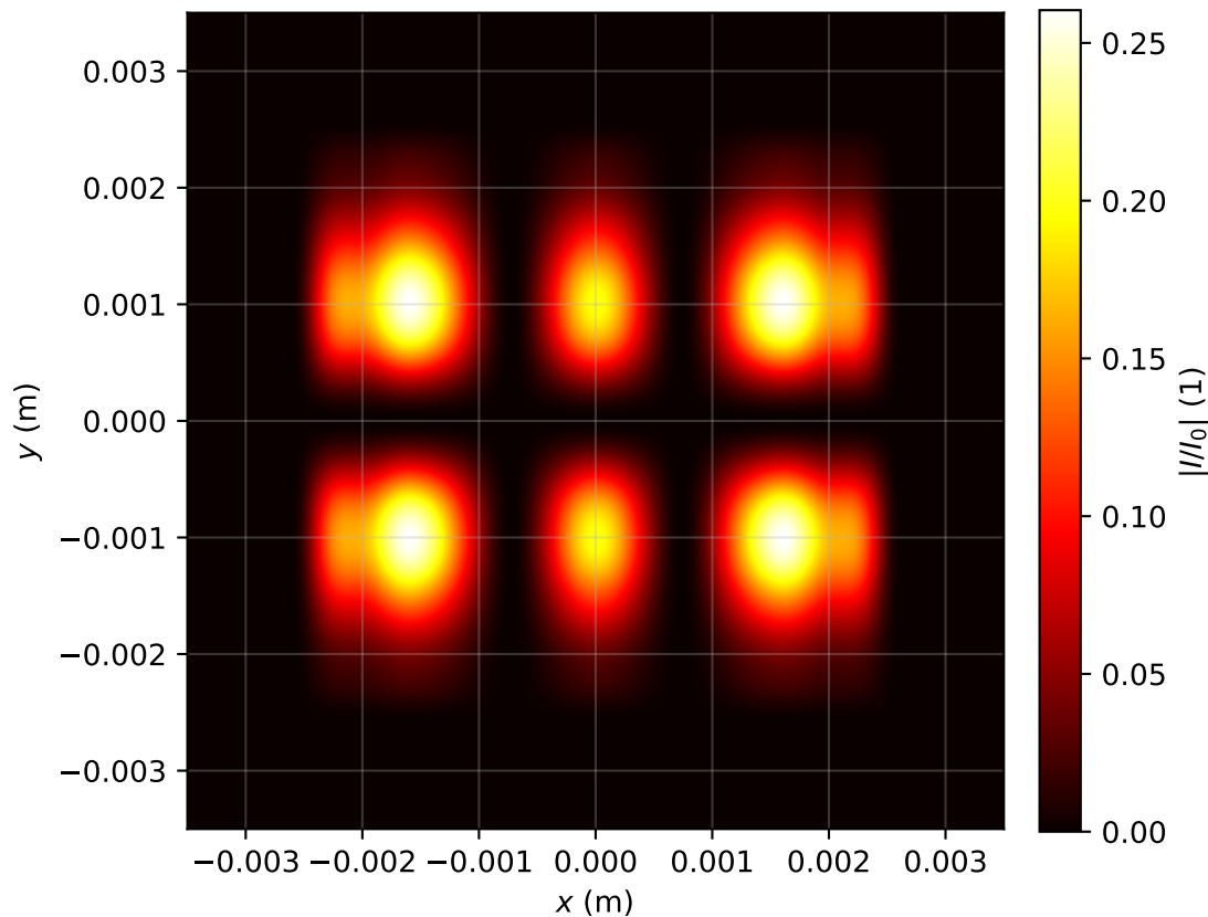
Intensity profile I(x, y, z = 3.582)/I_0 , P_{in}=0.5P_{cr} , artificial time
